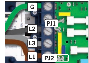
3-phase Delta (no neutral)
